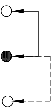
SCHEMATIC (NON-SHORTING)
