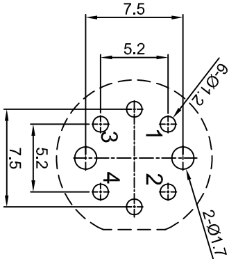
CIRCUIT
