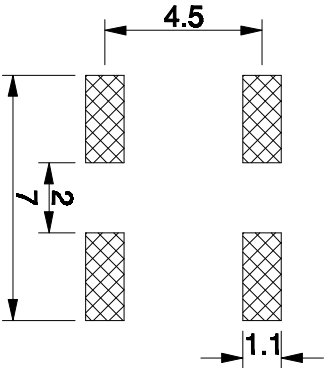
P. C. B LAYOUT
