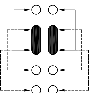
SCHEMATIC (SHORTING)
