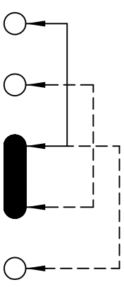
SCHEMATIC (SHORTING)
