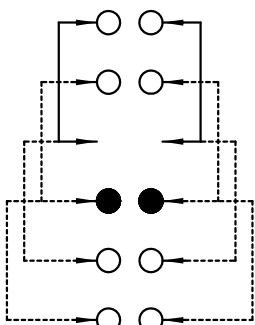
SCHEMATIC (SHORTING)
