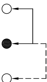
SCHMATIC (NON-SHORTING)
