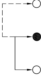
SCHEMATIC (NON-SHORTING)
