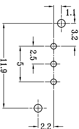
P.C.B LAYOUT BOTTOM VIEW
