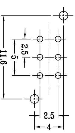
P.C.B LAYOUT BOTTOM VIEW
