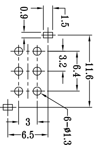
P.C.B LAYOUT BOTTOM VIEW
