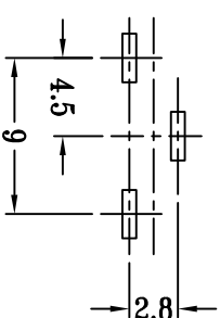
P.C.B LAYOUT BOTTOM VIEW
