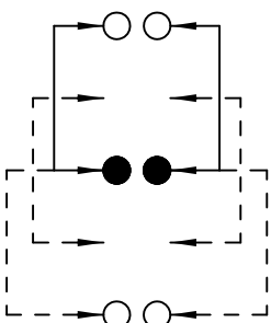
SCHEMATIC (NON-SHORTING)
