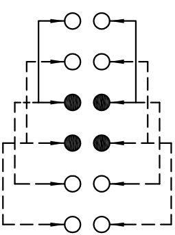
SCHEMATIC (SHORTING)
