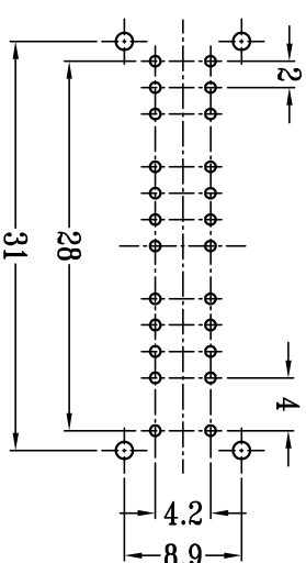
P.C.B LAYOUT BOTTOM VIEW
