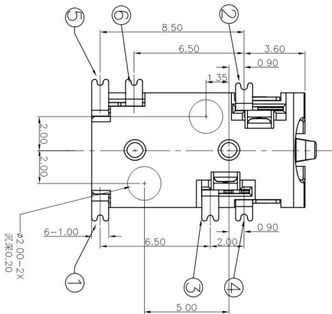
(ø3.50mm 4 POLE PLUG DETAIL DRAWING)
