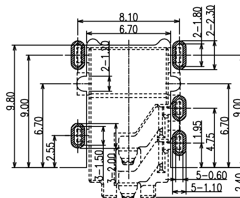
RECOMMENDED PCB LAYOUT(TOP VIEW) (GENERAL TOLERANCE0.05)
