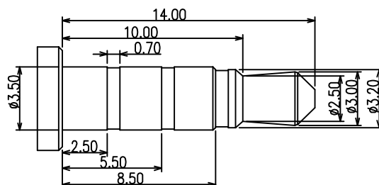
Ø3.50mm 4 POLE PLUG DETAIL DRAWING(2D)
