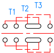
CIRCUIT
