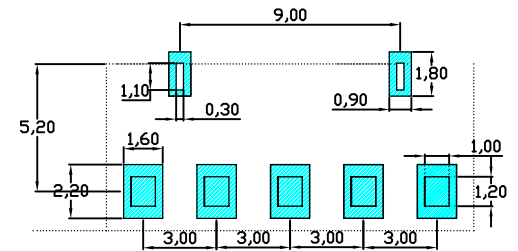
RECOMMENDED PCB LAYOUT TOP VIEW (.XX±0.05)
