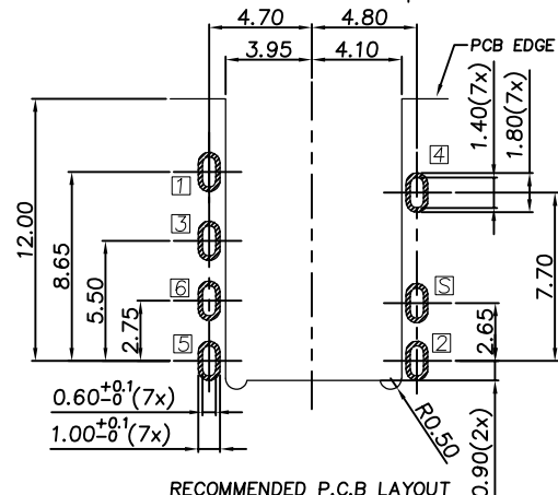
RECOMMENDED P.C.B LAYOUT TOP VIEW (TOLRANCE: \pm 0.05 )
