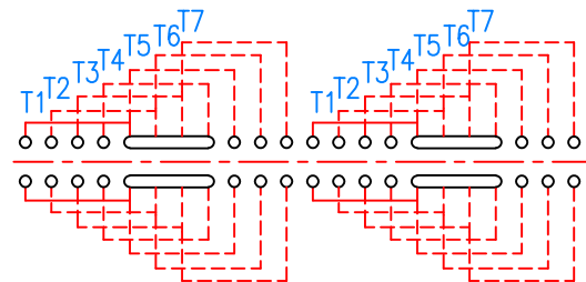
CIRCUIT
