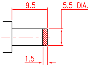
MATE PLUG
