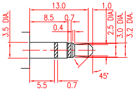
MATE PLUG
