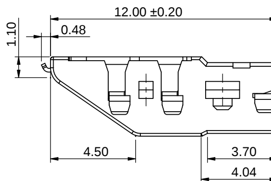
Ø 3.50mm 4 POLE PLUG DETAIL DRAWING(2:1)
