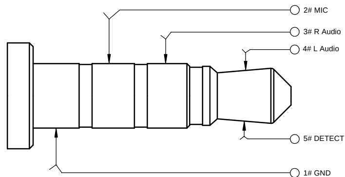
6 HOUSING HIGH TEMP BLACK _____ 5 TERMINAL 5 COPPER ALLOY _____ Au PLATED 4 TERMINAL 4 COPPER ALLOY _____ Au PLATED 3 TERMINAL 3 COPPER ALLOY _____ Au PLATED 2 TERMINAL 2 COPPER ALLOY _____ Au PLATED 1 TERMINAL 1 COPPER ALLOY _____ Au PLATED NO. DESCRIPTION MAT'L COLOR REMARK
