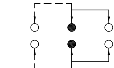
SCHEMATIC (NON-SHORTING)
