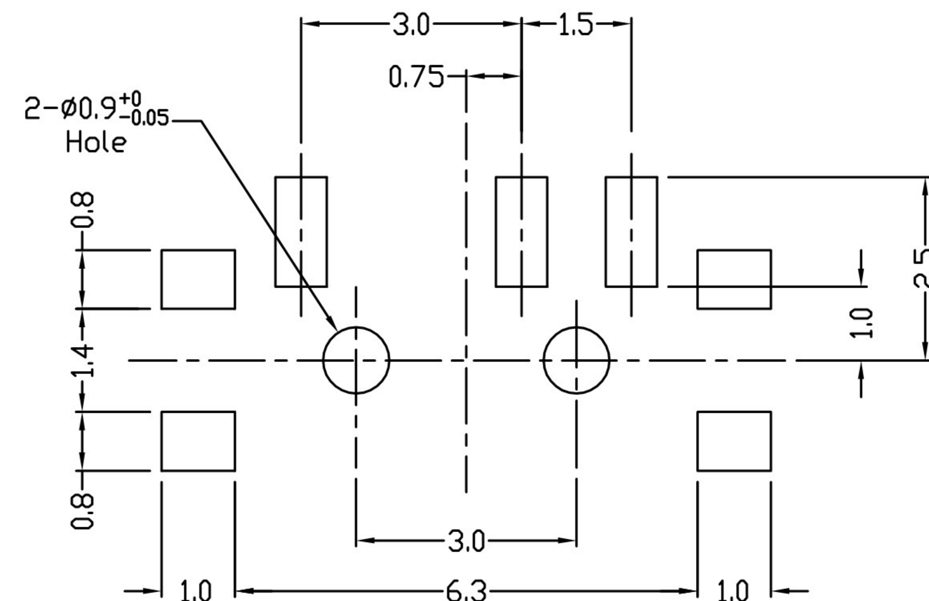
P.C. BOARD LAYOUT VIEW A
