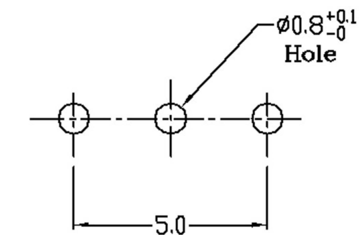
P.C. BOARD LAYOUT
