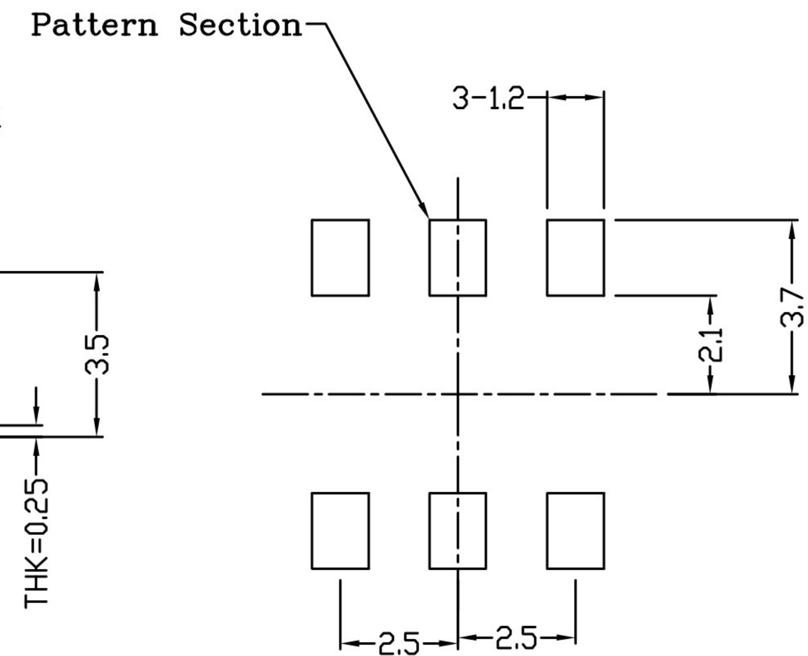
P.C. BOARD LAYOUT
