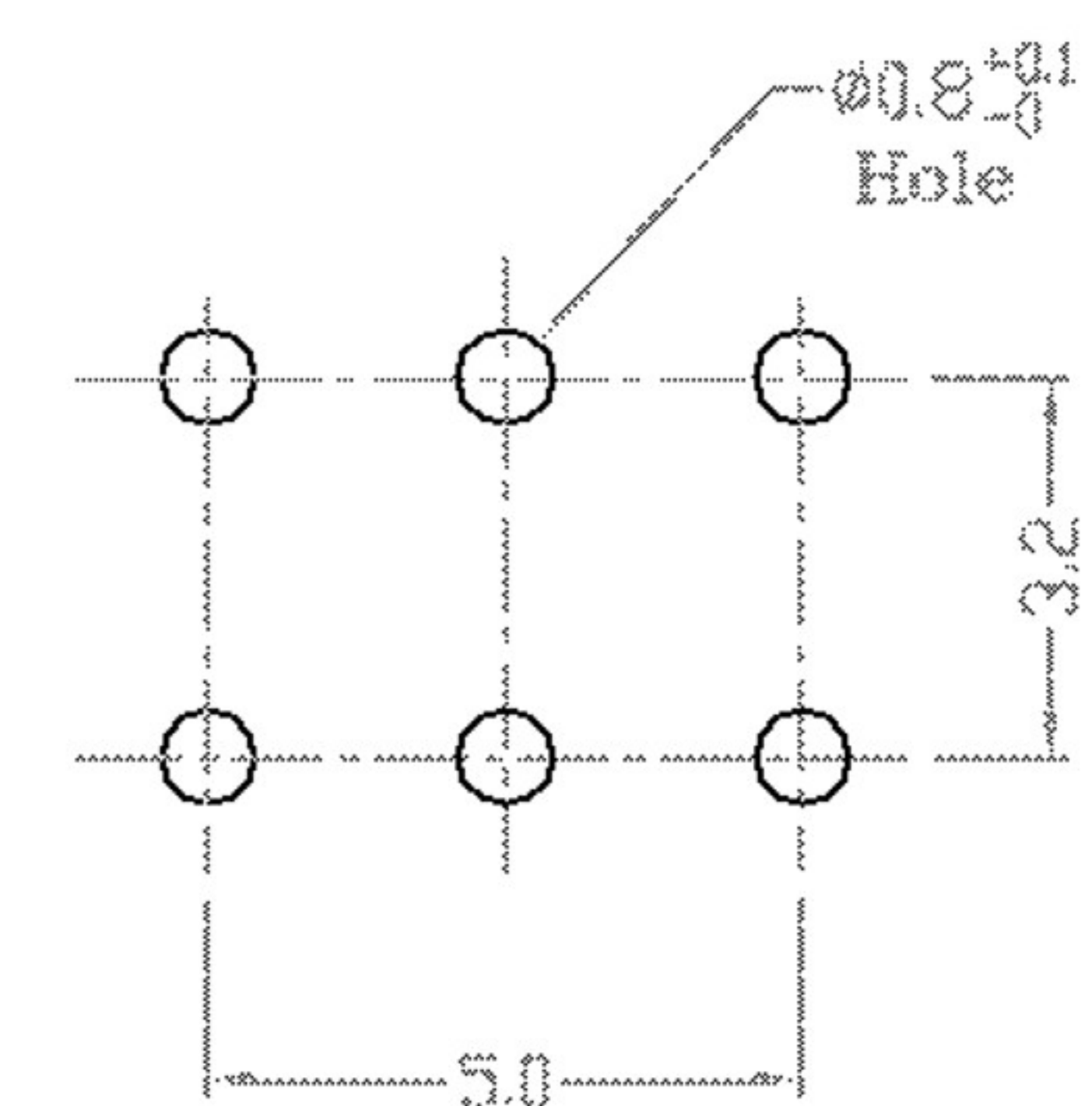
P.C. BOARD LAYOUT
