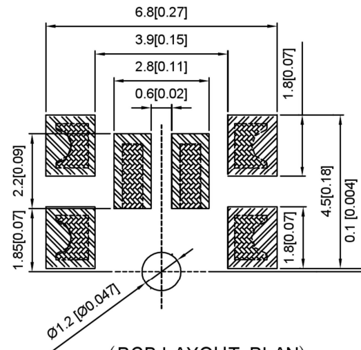
(PCB LAYOUT PLAN)
