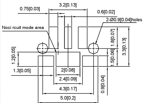
PCB MOUNTING DRAWING
