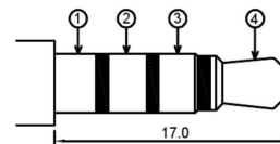
Ø3.50mm 4 POLE PLUG
