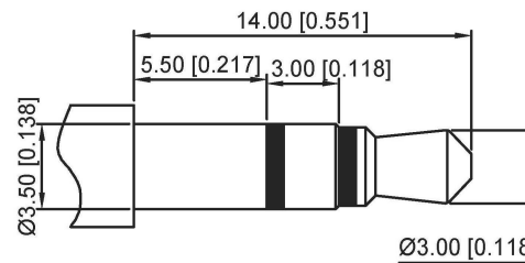
Ø3.50mm 3 POLE PLUG
