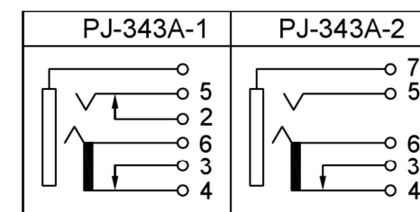
SCHEMATIC
