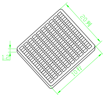
吸塑盒 (200pcs)
