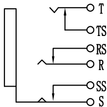
Electrical schematic
