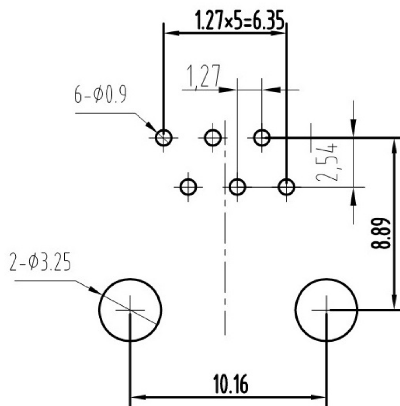
PC Board Layout Component Side Shown
