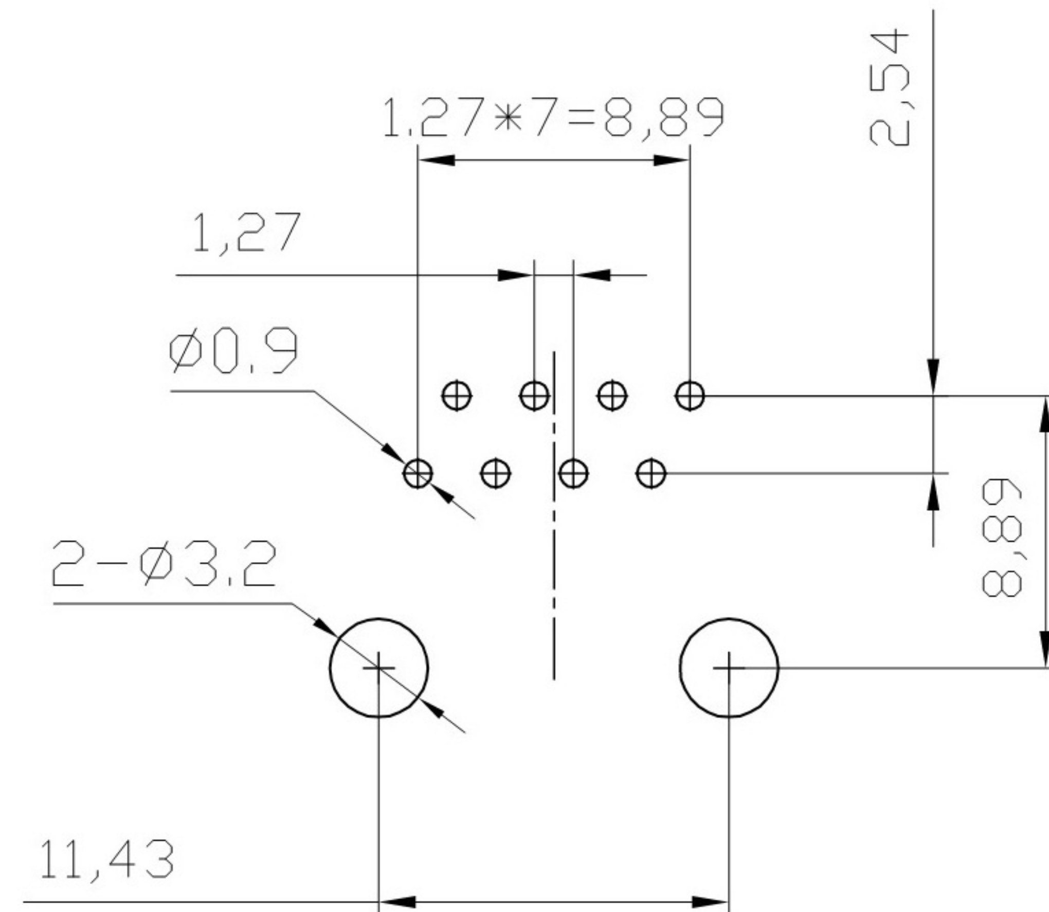
PC Board Layout Component Side Shown
