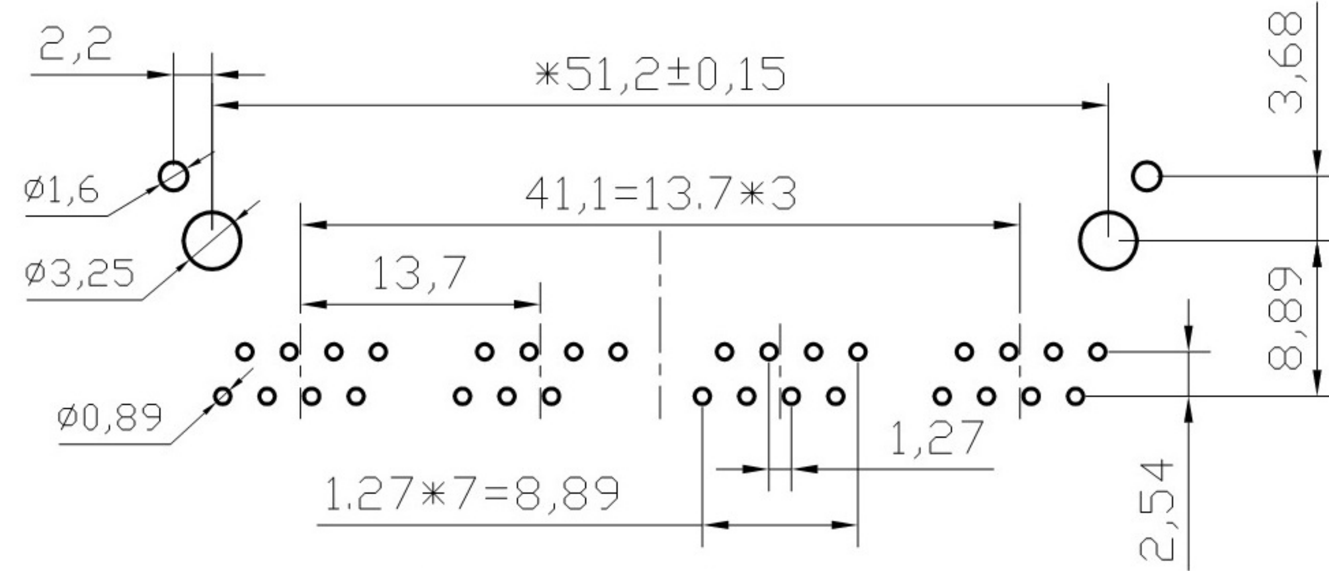
PC Board Layout Component Side Shown
