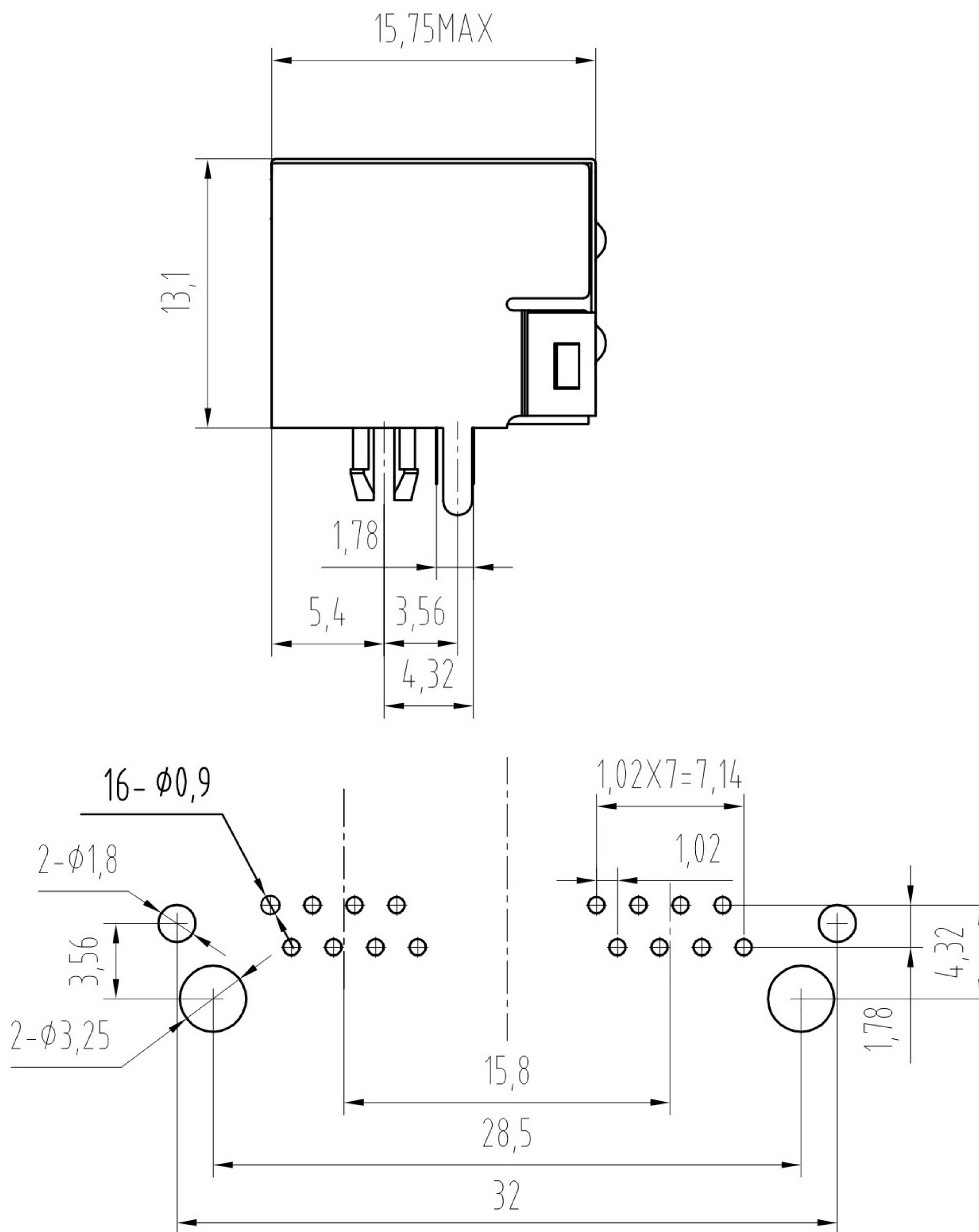
PC Board Layout Component Side Shown
