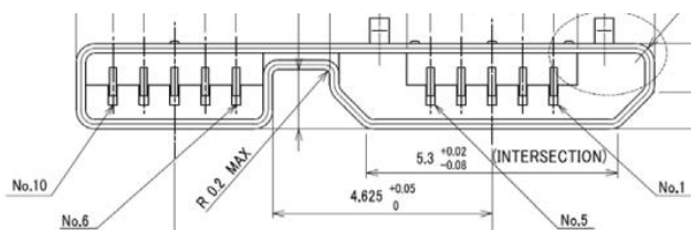
USB 3.0 Micro B Plug
