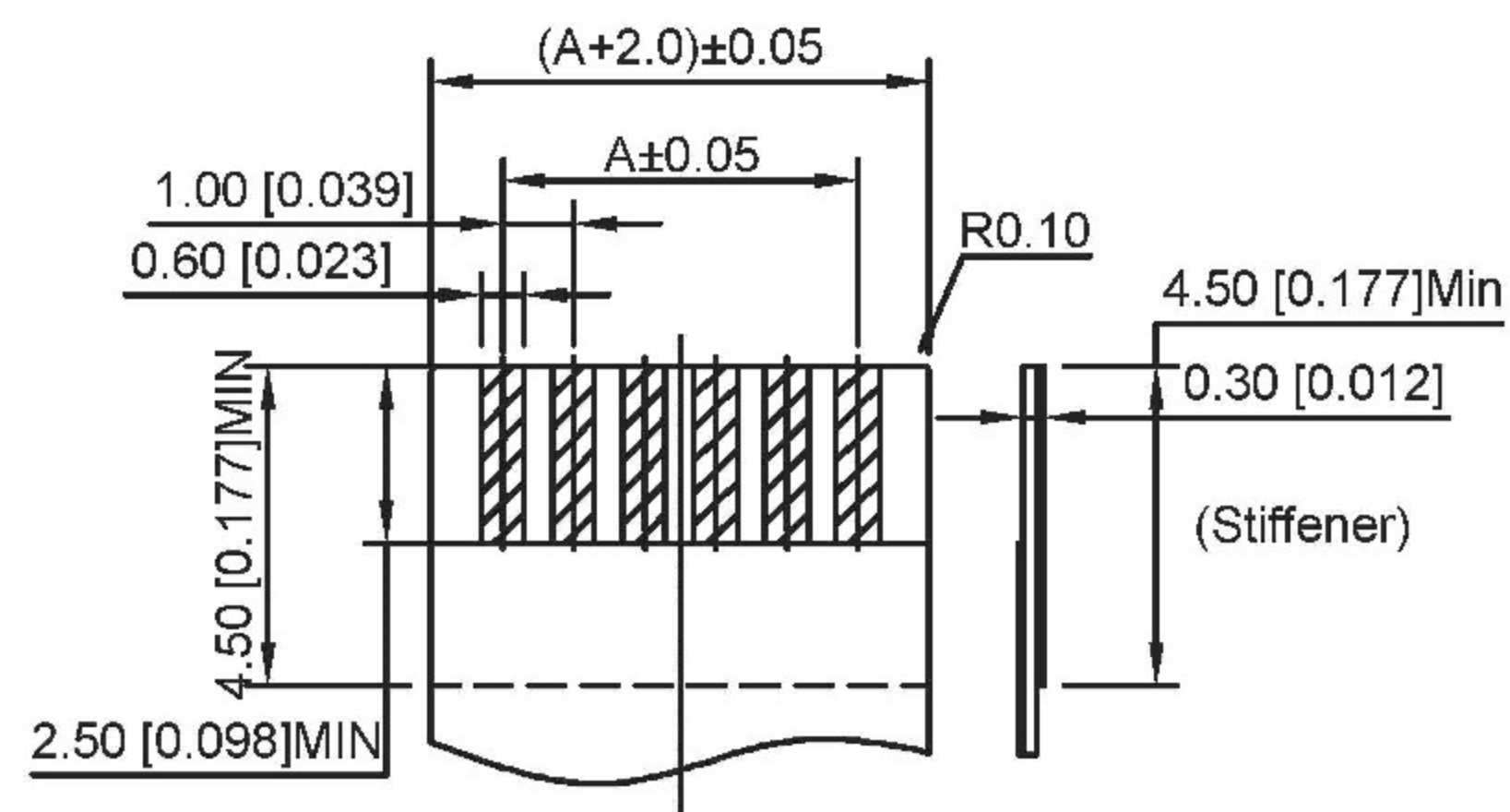
RECOMMENDED FFC/FPC
