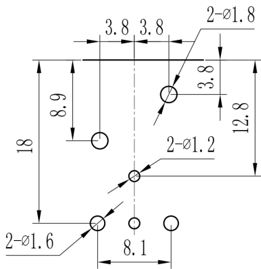
P. C. B LAYOUT (BOTTOM VIEW) Tolerance: ±0.05
