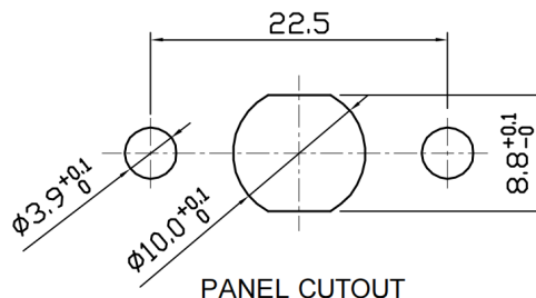
PANEL CUTOUT
