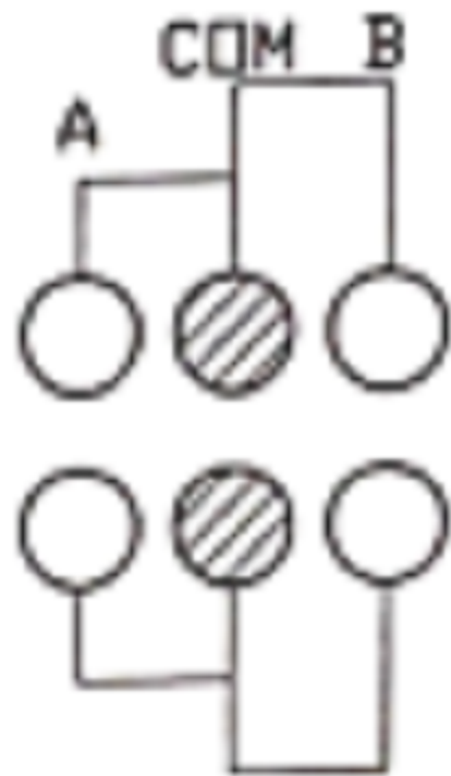
SCHEMATI (2P2)
