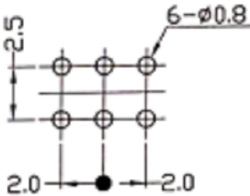
PIERCING PLAN
