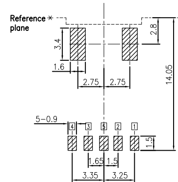
Recommended PCB Layout Tolerance: ±0.1(Top view)
