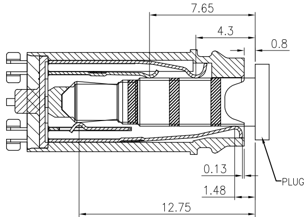
SEC:A-A Image of plug match with contact point
