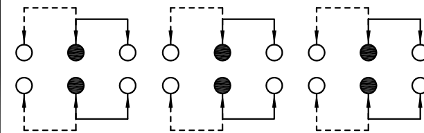
SCHEMATIC (NON-SHORTING)
