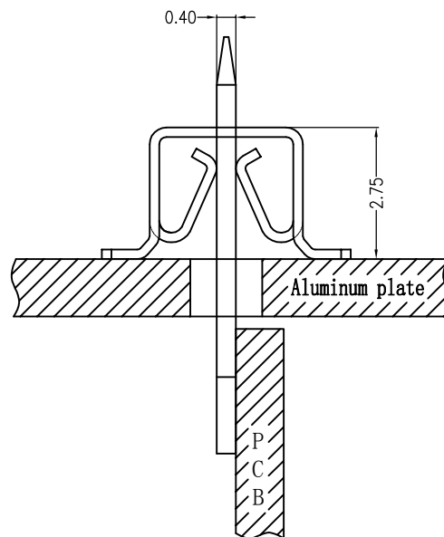
Assembly Layout
