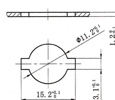
安装开孔尺寸 MOUNTING HOLE DIMENTION
